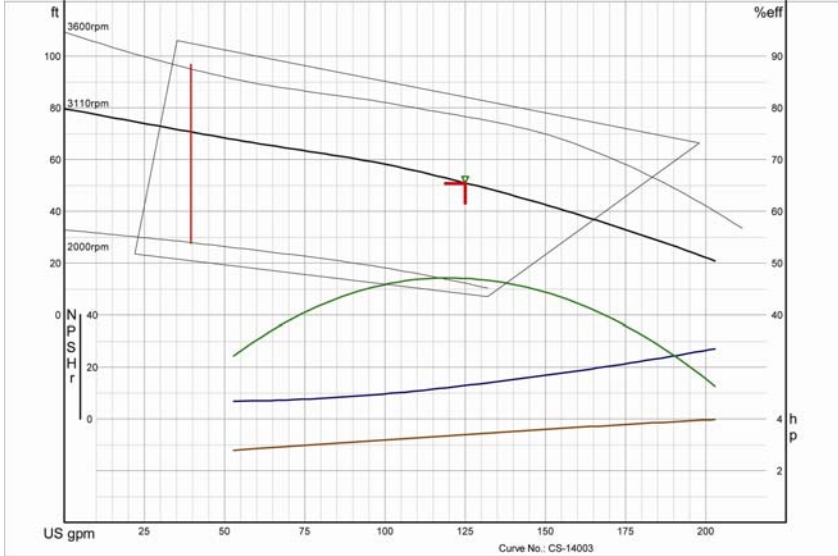
American-Marsh Pumps 08/20/05 Model: 125 GPM Water Pump Size: 2x2-5 SPHE Speed: 3110 rpm
